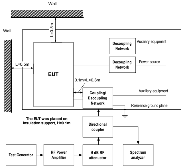
Photograph 9.5.2 Setup for immunity to conducted disturbances induced by radio frequency fields at telecommunication line, CDN injection method
