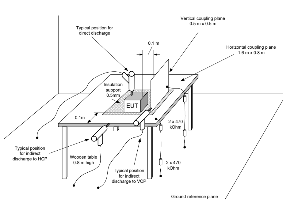
Figure 9.1.1 Setup for immunity to ESD, table-top EUT
