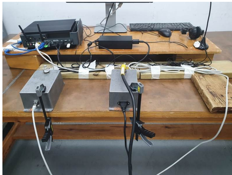
Photograph 9.5.1 Setup for immunity to conducted disturbances induced by RF fields at AC power supply line
