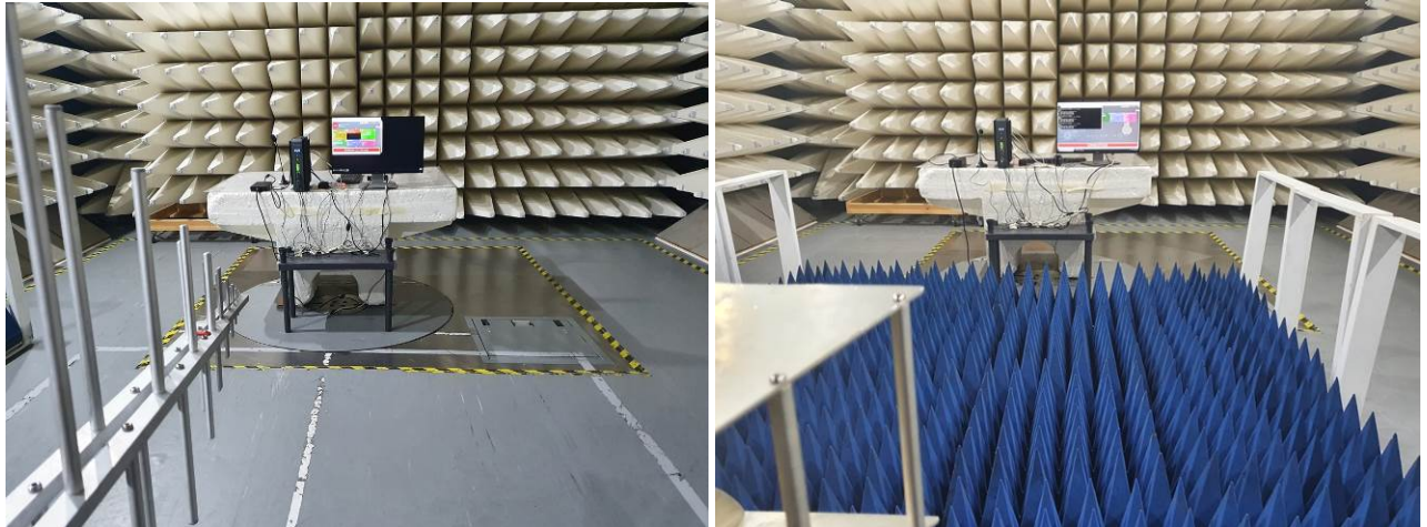
Photograph 8.3.2 Setup for radiated emission measurements, EUT cabling
