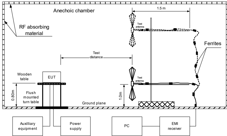
Figure 8.3.1 Setup for radiated emission measurements in semi anechoic chamber below 1 GHz, table-top EUT
