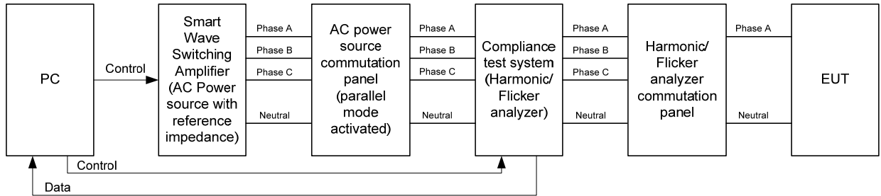
Figure 8.4.1 Setup for harmonic current emissions test
