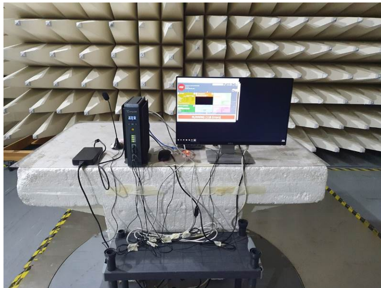
Photograph 8.3.2 Setup for radiated emission measurements, EUT cabling
