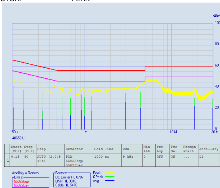
Plot 8.1.2 Conducted emissions at AC mains power port, AC mains input of AC/DC adapter
