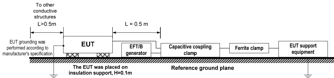
Photograph 9.3.2 Setup for conducted immunity to EFT/B at telecommunication line
