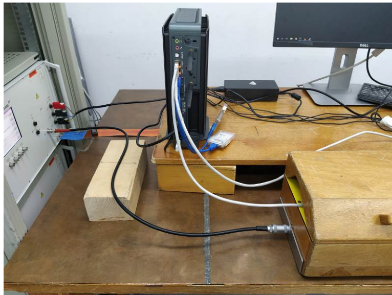
Photograph 9.3.2 Setup for conducted immunity to EFT/B at telecommunication line
