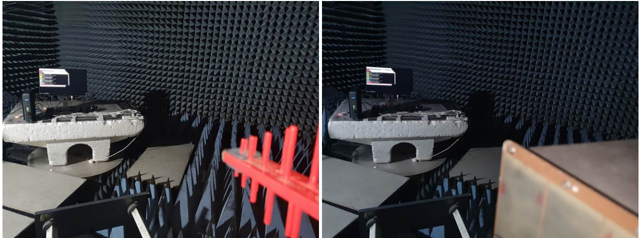
Photograph 9.2.2 Setup for radiated immunity to RF electromagnetic field test, EUT cabling
