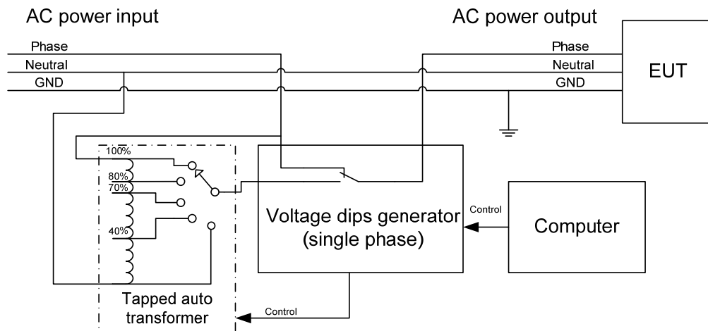
Figure 9.7.1 Setup for immunity to voltage dips and short interruptions test
