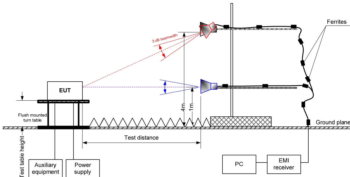
Figure 7.2.2 Setup for radiated emission measurements in semi anechoic chamber in 1000 – 26000 MHz range, table-top EUT
