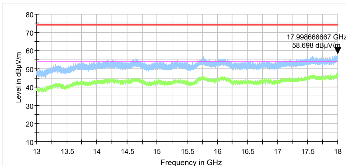
Plot 7.2.2 Radiated emission measurements in 18 - 26 GHz range, vertical and horizontal antenna polarization
