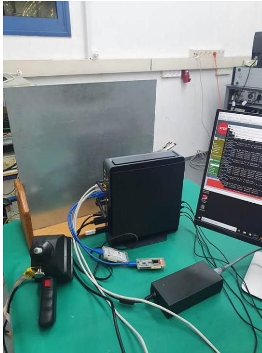
Photograph 9.1.2 Setup for immunity to ESD, EUT test points
