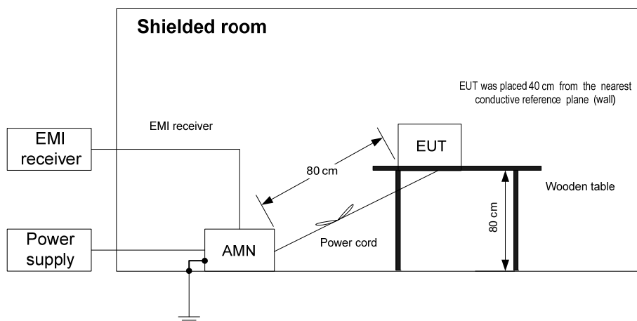
Figure 8.1.1 Setup for conducted emission measurements at AC mains power port, table-top EUT
