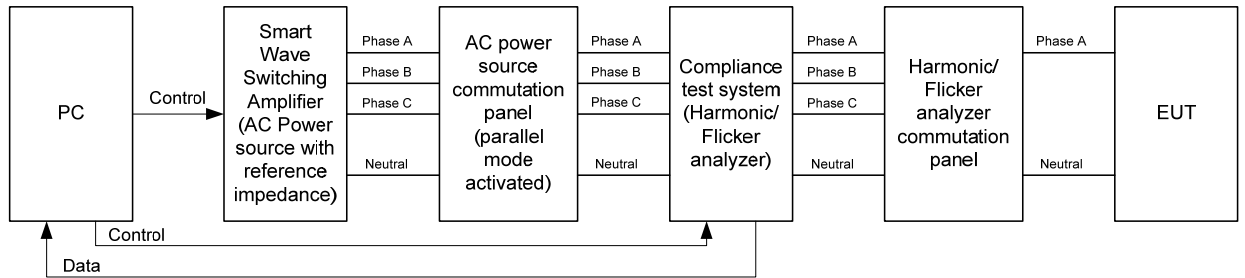
Figure 8.5.1 Setup for voltage fluctuations and flicker test
