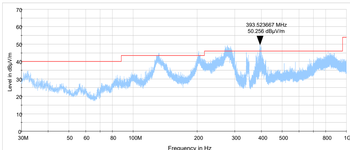
Plot 7.2.2 Radiated emission measurements in 1 - 13 GHz range, vertical and horizontal antenna polarization
