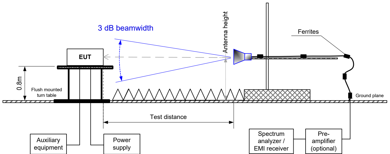
Figure 8.3.2 Setup for radiated emission measurements in semi anechoic chamber above 1 GHz, table-top EUT
