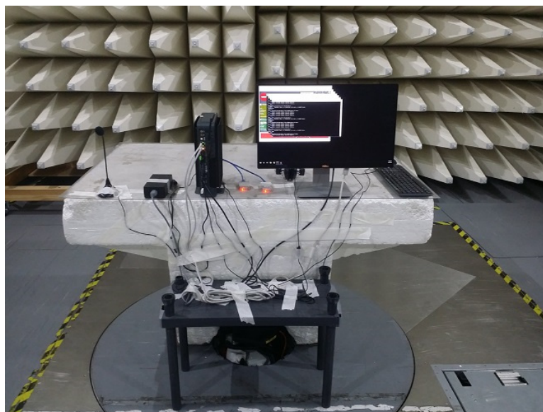
Photograph 7.2.2 Setup for radiated emission measurements, EUT cabling
