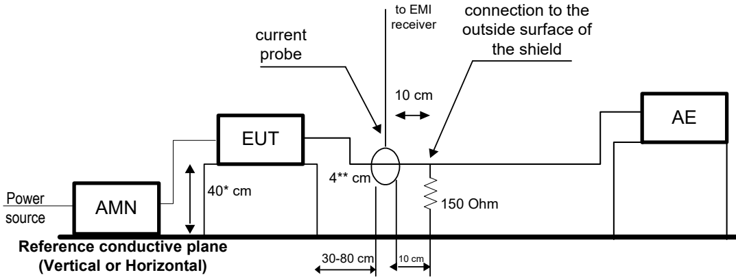
Figure 8.2.1 Setup for conducted emission measurements at wired network ports with current probe
